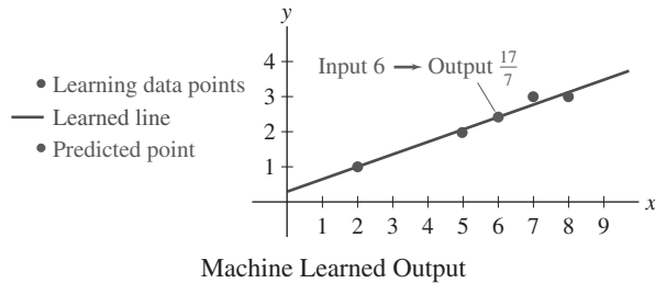
FIGURE 3 Machine-learned output.
