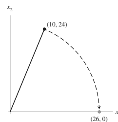
A Givens rotation in \mathbb{R}^2 .
